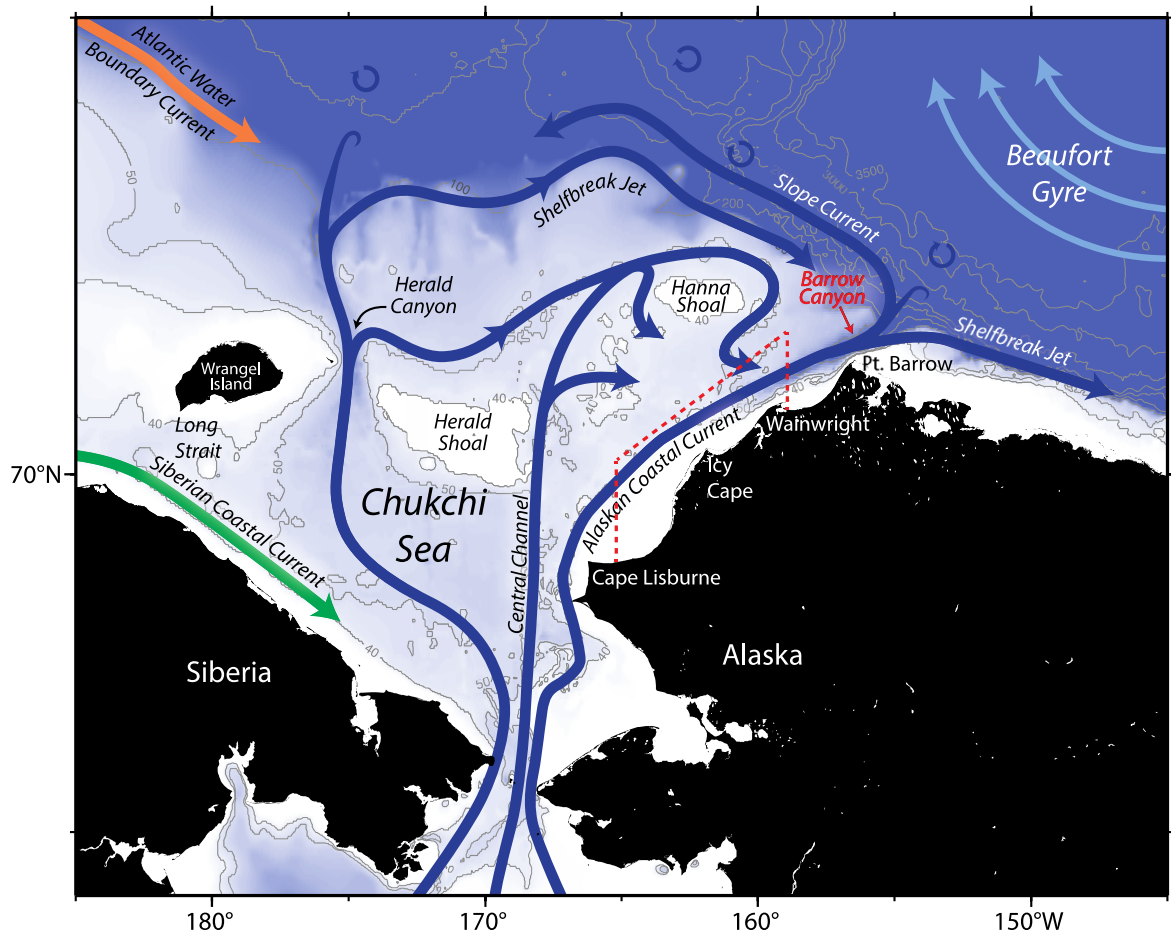
1002 1003 Figure 1. Schematic circulation of Pacific-origin water in the Chukchi Sea and geographical place names (adopted from 1004 Corlett and Pickart, 2017). The polynya box in the northeast part of the shelf, discussed in Section 4.2, is delimited by 1005 the dashed red line.
