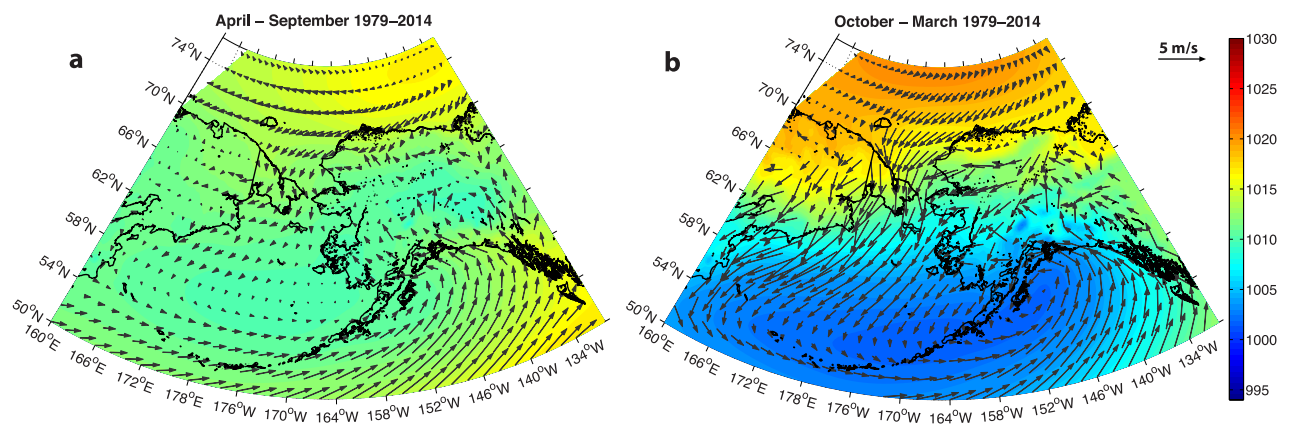
Figure 6. Maps of climatological mean sea level pressure (mb, color) and 10m winds (vectors) from NARR for the period 1979–2014. (a) the warm season (April–September); (b) the cold season (October–March).
