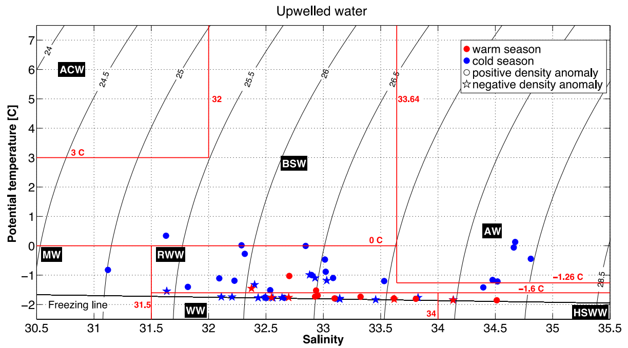
Figure 10. The T/S value of the water measured by the mooring at the peak of each upwelling event. Red symbols are the events during the warm season, and blue symbols are the events during the cold season. Circles (stars) denote events associated with positive (negative) density anomaly. The water mass definitions are the same as in Figure 3.
