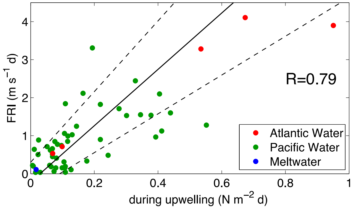
Figure 14. Value of FRI versus I_w for upwelling events (circles), and the linear fit (black line). The 99% significant levels are indicated by the dashed lines. The color of the symbols (red, green, blue) mark the water type present at the peak of each event (Atlantic water, Pacific origin water, meltwater respectively).
