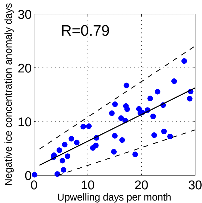
Figure 15. Number of upwelling days per month versus the number of negative ice concentration anomaly days in the polynya box of Figure 1 (see text for details). The linear fit is shown (black line) along with the 99% significance levels (dashed lines).
