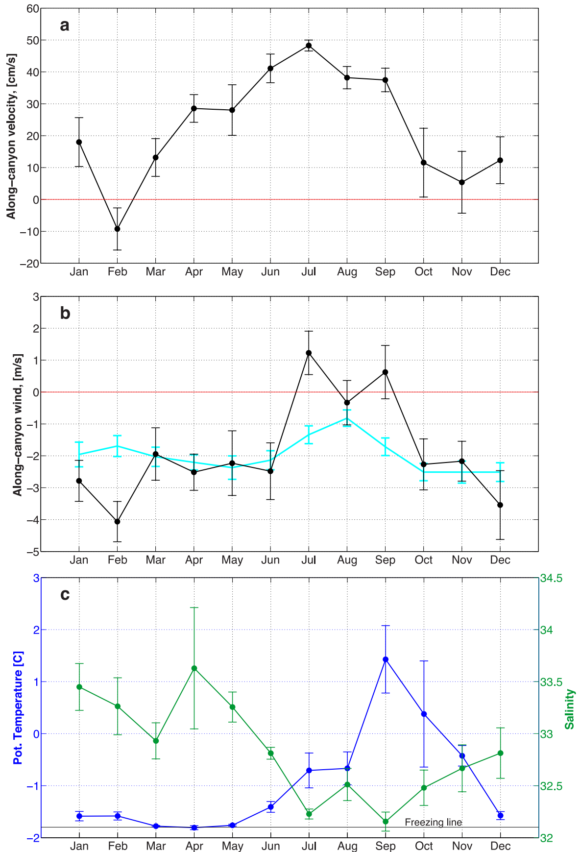
Figure 4. (a) Monthly means and standard errors for the along-canyon component of the velocity from the mooring near the head of Barrow Canyon deployed from 2002–4. (b) Same as (a) for the along-canyon component of the wind at Barrow for the mooring deployment period (black curve) and for the climatological period 1979–2014 (cyan), with the standard errors indicated by the bars. Positive values are down-canyon flow/wind. (c) Same as (a) for the potential temperature (blue) and salinity (green) from the mooring. The freezing line is shown in black.
