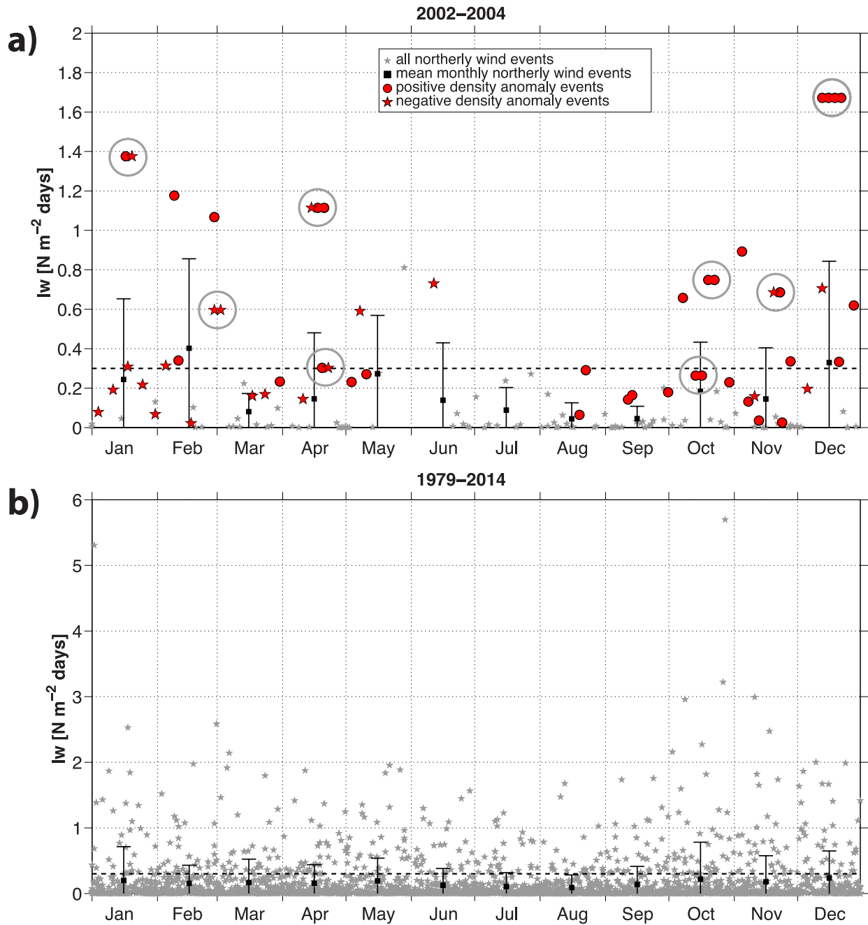
Figure 13. Time integral of the wind stress I_w for the up-canyon wind events for (a) the mooring deployment period 2002–4, and (b) the climatological period 1979–2014. The grey stars are the individual events and the black squares are the monthly means. The standard deviations are denoted by the bars. In (a) those events associated with upwelling are indicated by the red circles (positive density anomaly events) and the red stars (negative density anomaly events). The open circles denote multiple upwelling events corresponding to a single storm. The threshold of I_w = 0.3 \text{ N m}^{-2} \text{ d} is shown by black dashed line. Note: for presentation purposes the absolute value of I_w is plotted (since it is a negative quantity for northeasterly wind events).
