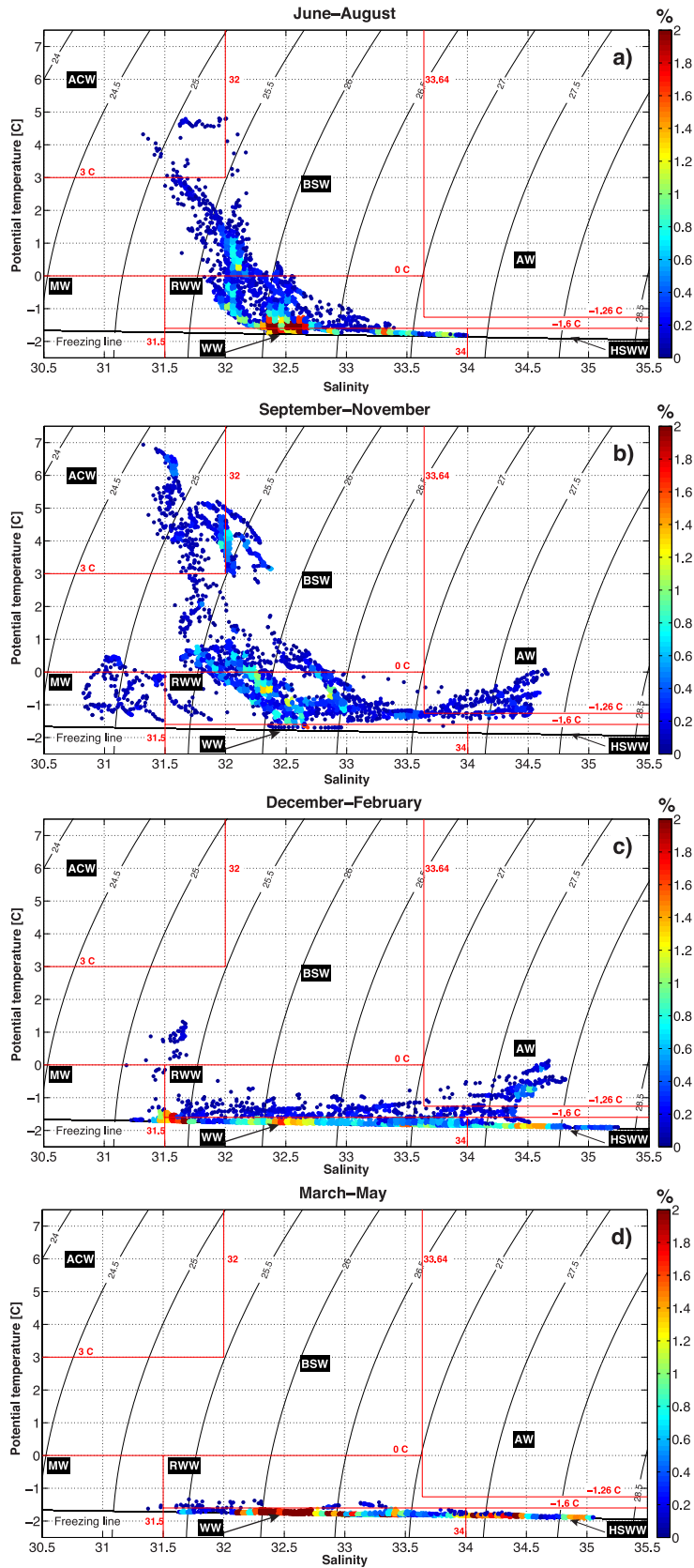
Figure 3. Seasonal T/S diagrams for the water measured by the mooring, where the color represents the percentage of occurrence of the measurements within bins of 0.05^{\circ}\text{C} in potential temperature by 0.2 in salinity. (a) June – August; (b) September – November; (c) December – February; and (d) March – May. The water mass boundaries are denoted by the red lines. ACW = Alaskan coastal water; BSW = Bering summer water; WW = newly ventilated Pacific winter water; RWW = remnant Pacific winter water; HSWW = hypersaline Pacific winter water; MW = Arctic-origin meltwater / river discharge water; and AW = Atlantic water.
