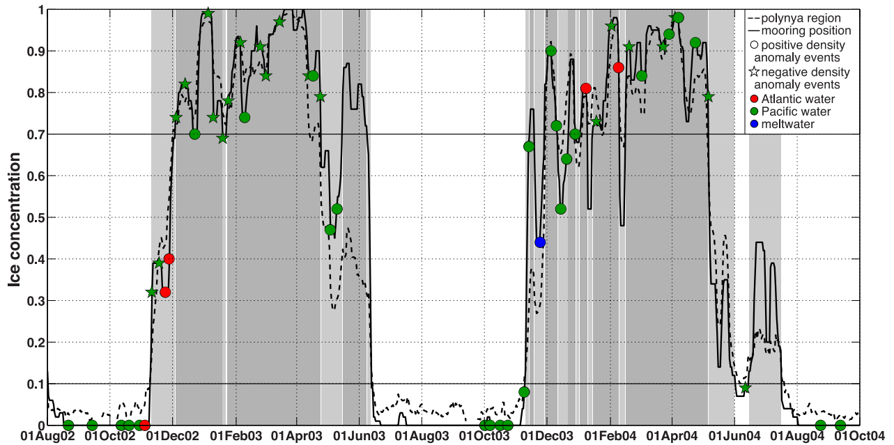
Figure 8. Ice concentration at the mooring site (solid black line) and median ice concentration within the polynya box (dashed black line) during the two-year mooring deployment (see Figure 1 for the location of the polynya box). The circles (stars) mark the positive (negative) density anomaly events. The color of the symbols (red, green, blue) mark the water type present at the peak of each event (Atlantic water, Pacific origin water, meltwater respectively). The shading indicates the three ice seasons: open water (white), partial ice cover (light grey), and full ice cover (dark grey).
