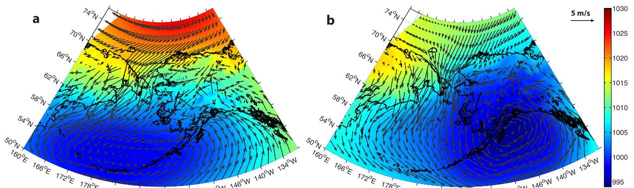
Figure 9. Composite average maps of sea level pressure (mb, color) and 10m winds (vectors) from NARR for (a) periods when upwelling occurred along the Beaufort slope as well as at the head of Barrow canyon, and (b) periods when upwelling occurred only in the canyon.
