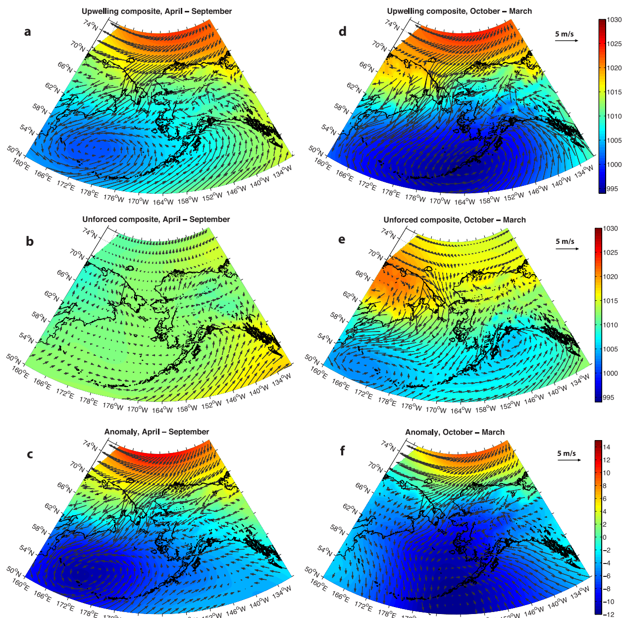
Figure 11. Maps of sea level pressure (mb, color) and 10m winds (vectors) from NARR for periods of upwelling (a and d) versus non-forced periods (b and e), along with the anomalies (upwelling minus non-forced, c and f). Left panel (a, b, c): the warm season (April–September); right panel (d, e, f): the cold season (October–March).
