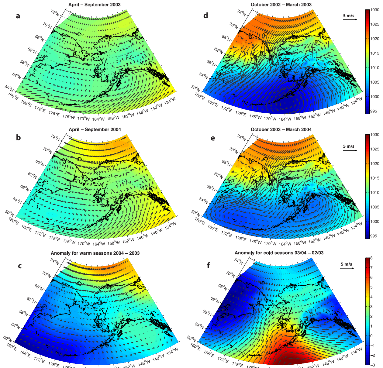
Figure 7. Maps of sea level pressure (mb, color) and 10m winds (vectors) from NARR for the warm and cold season of each mooring deployment year, along with the anomaly fields. Left panel (a, b, c): the warm season (April–September); right panel (d, e, f): the cold season (October–March).
