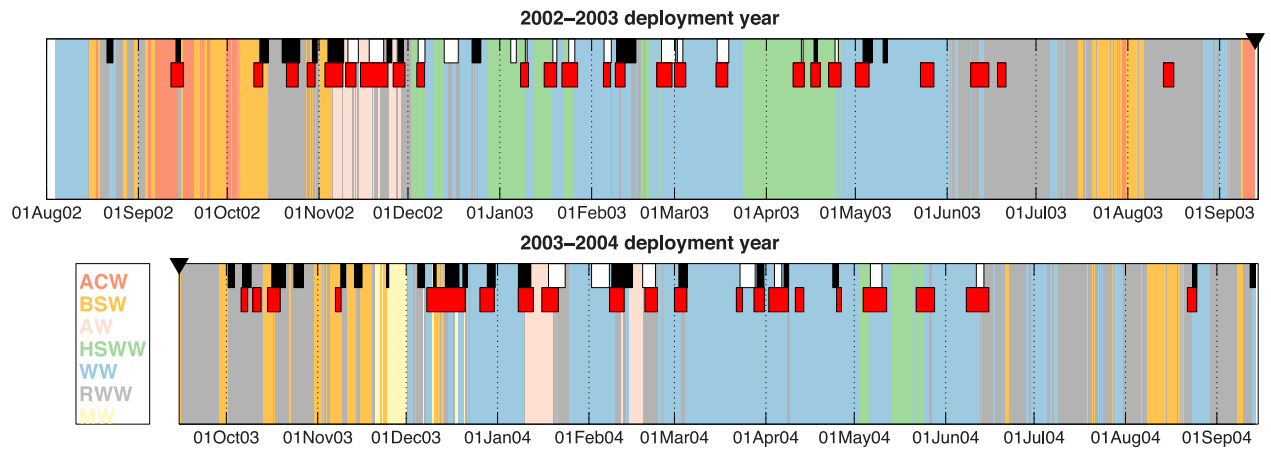
Figure 5. Time series of water masses using the temperature and salinity data from the mooring at the head of Barrow Canyon. The top panel is the 2002–3 deployment, and the bottom panel is the 2003–4 deployment. The mooring turnaround date is denoted by the black triangle in each panel. The different water masses are indicated by the different colors (see the legend). The water mass abbreviations are defined in the caption of Figure 3. The upwelling events at the head of Barrow Canyon are indicated by the black (positive density anomaly events) and white (negative density anomaly events) patches at the top of each panel. The upwelling events at the Beaufort Slope (Schulze and Pickart, 2012) are indicated by red patches (positive density anomaly events).
