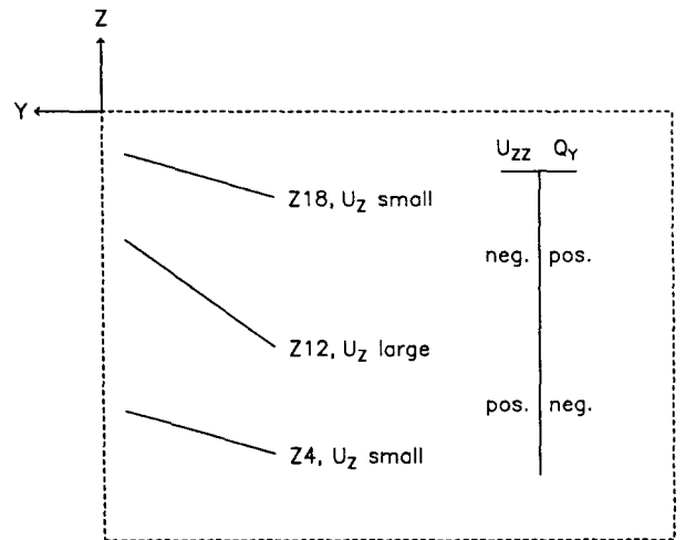
FIG. 12. (a) Temperature section across the Gulf Stream (from Pickart et al. 1992b). (b) Schematic illustrating the increased isotherm slope of the central thermocline in (a) and its implications (by thermal wind) on the meridional gradient of potential vorticity Q .
