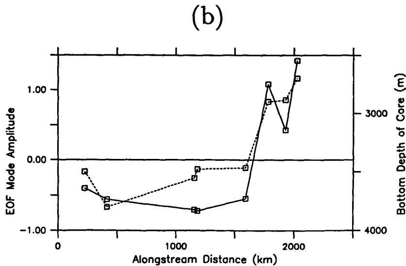
FIG. 12. (a) Vertical structure of EOF mode 1 for the normalized oxygen sections, accounting for 65% of the total variance. (b) Mode amplitude versus alongstream distance (solid line) compared to bottom depth of the DWBC core (dashed line).
